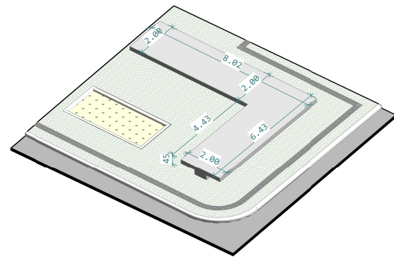
3 BANCO CONCRETO
